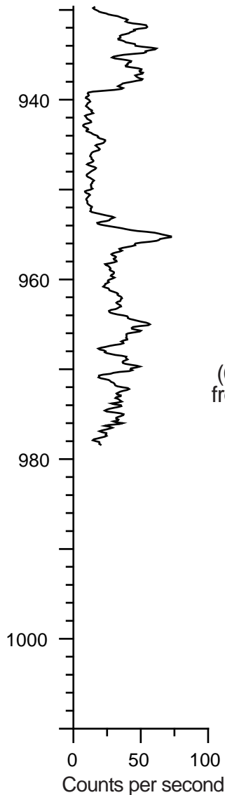
Natural Gamma Log
